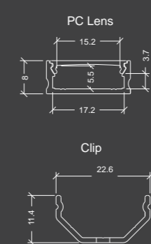
Sectional Dimensions (mm)
