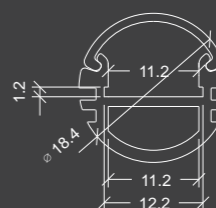
Sectional Dimensions (mm)
