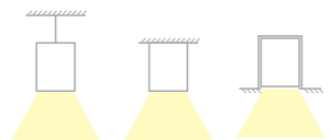
Suspndent installation Ceiling installation Embedded Installation
