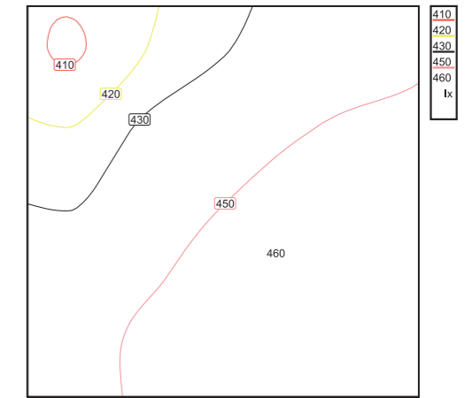
Scale: 1 : 10 Horizontal illuminance (Grid) Average: 446 lx, Min: 409 lx, Max: 475 lx, Min/average: 0.917, Min/max: 0.861, Points: 5 x 5 (Relevant: all)
