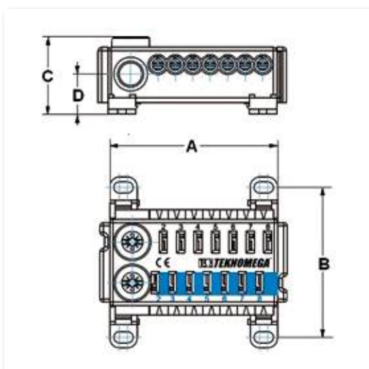
RPU5000
