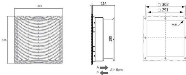
Fan and filter FK 5528.230
